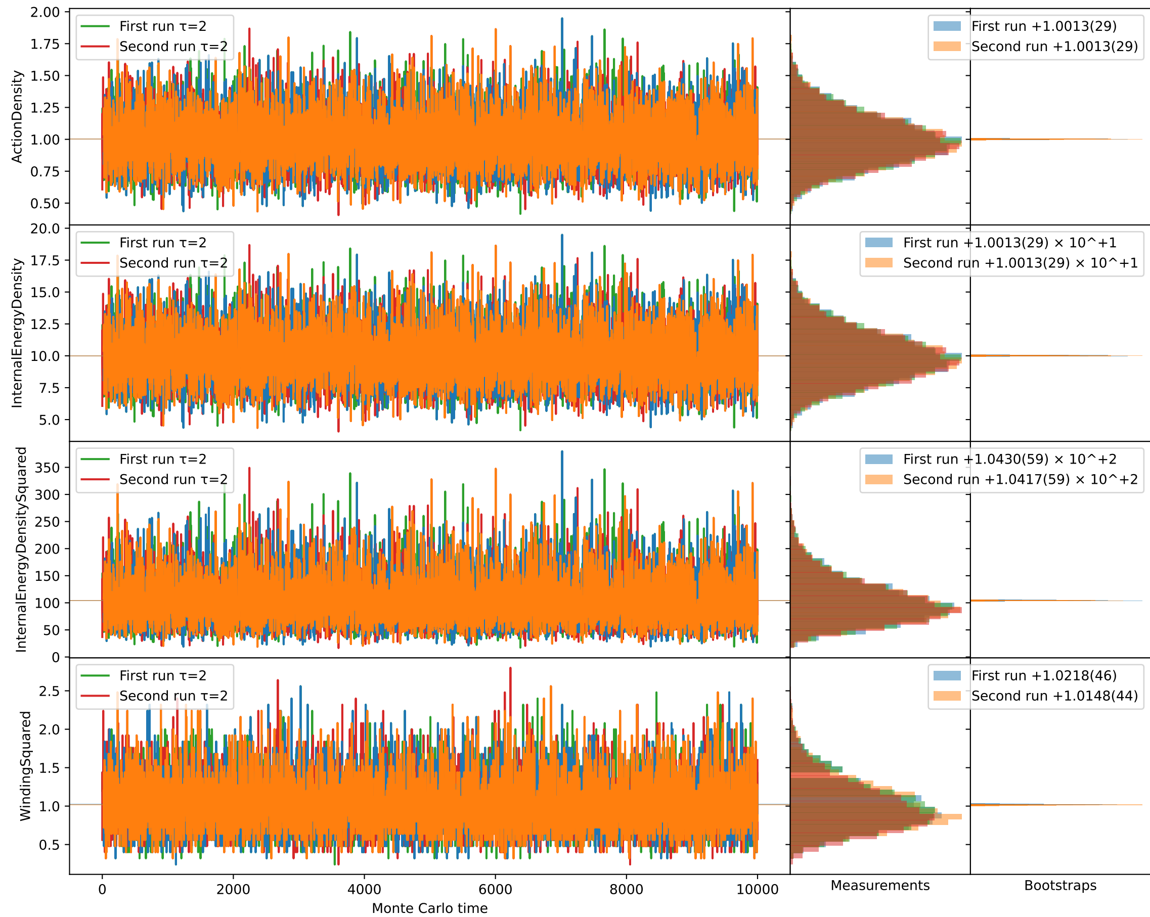
Villain N=5 \kappa=0.1 W=1
