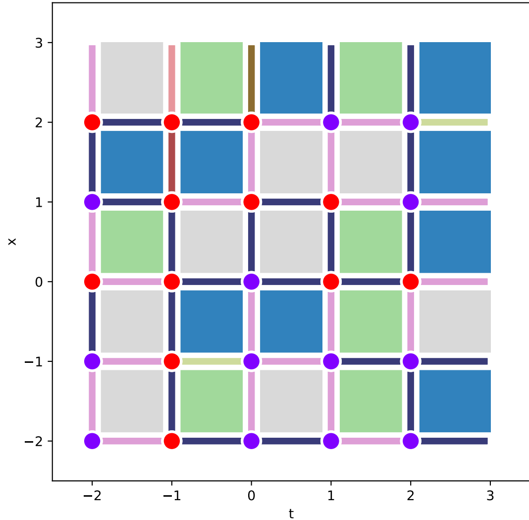
Villain(Lattice2D(5,5), \kappa=0.1 , W=1 )
